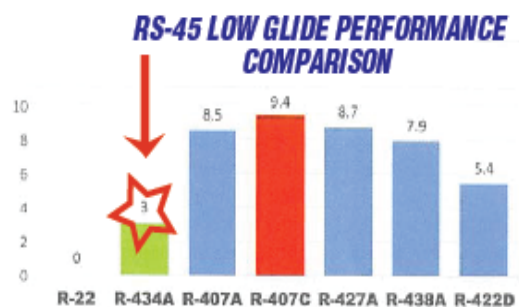
Comparison of glide for common R22 alternatives at the same conditions. Flooded systems require ultra low glide refrigerants.
